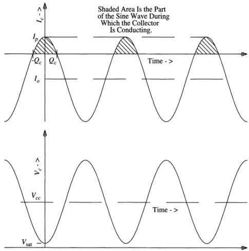
Figure 7.8 Voltage and current waveforms for Figure 7.7. [R. Weber, Microwave Engineering Course Notes , ©1987–1997, August 1997 edition, p. 68.]
