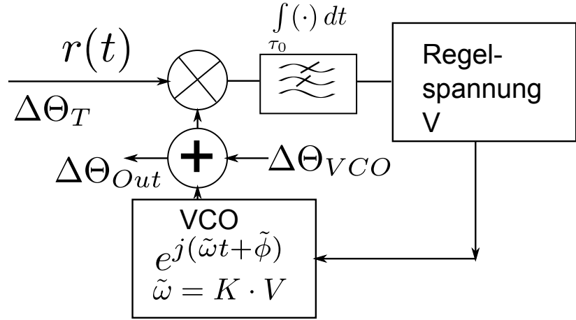
Generic Phase locked loop
