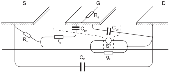
Pictorial derivation of equivalent circuit for a MESFET
