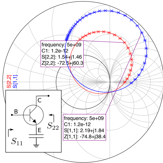
Source-feedback drives S_{11}, S_{22} in Circles
