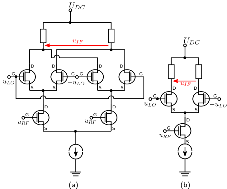
Gilbert Cell (Double Balanced Mixer) (a), single balanced mixer (b)
