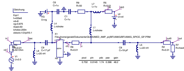
Schematic for Class-A amplifier based on NXP's BFU590G BJT
