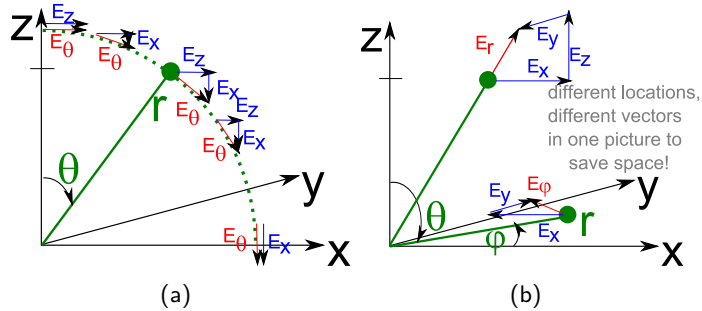
(a) Vector with only \theta -component at different locations in x-z- ( \phi = 0 or \theta )-plane, (b) One vector with \phi -components in x-y ( \theta = \pi/2 or \phi )-plane and another vector at another location with only r - (radial) component
