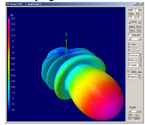
yagi 15
