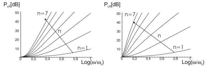
(a) Butterworth, (b) Chebycheff.
