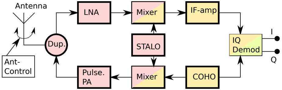
(Mostly) Analog part of a typical pulse Radar
