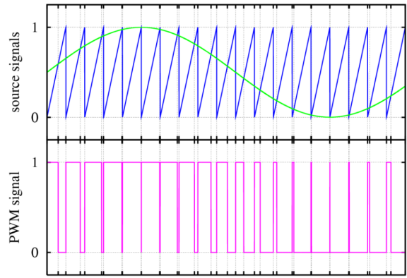
Pulse-width-modulation as input for switching amplifier
