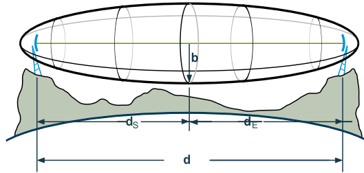
Fresnel ellipsoid (source: Wikipedia (modified), GPLD)
