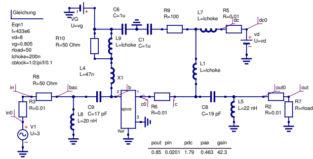
Schematic for Class-B amplifier based on NXP's BJT
