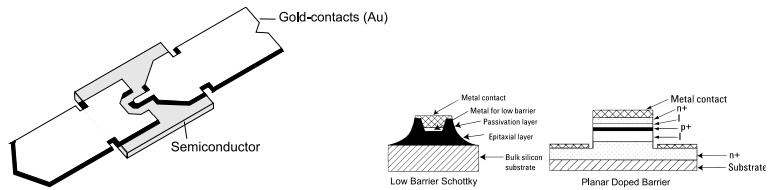
(a) Beam-lead technology for high frequency (it's all about packaging), (b) Epitaxial layers
