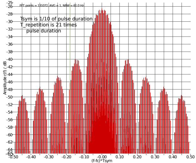
Spectrum of a repeated pulses, observe overlay of \sin(x)/x and comb pattern
