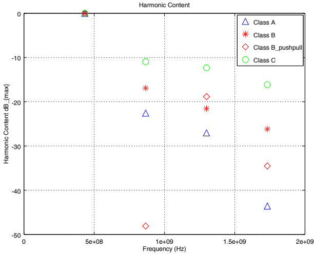
Comparison of harmonic content in output signal. Simulation engine: Xyce (Serial) via QUCS
