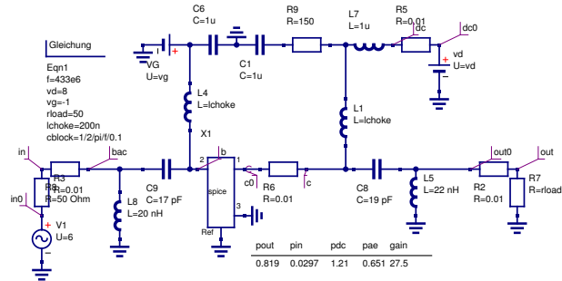
Schematic for Class-C amplifier based on NXP's BJT
