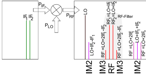
Mixer performance/ spectrum with two tones at input
