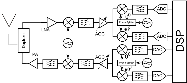
Block-diagram of a typical transceiver circuit
