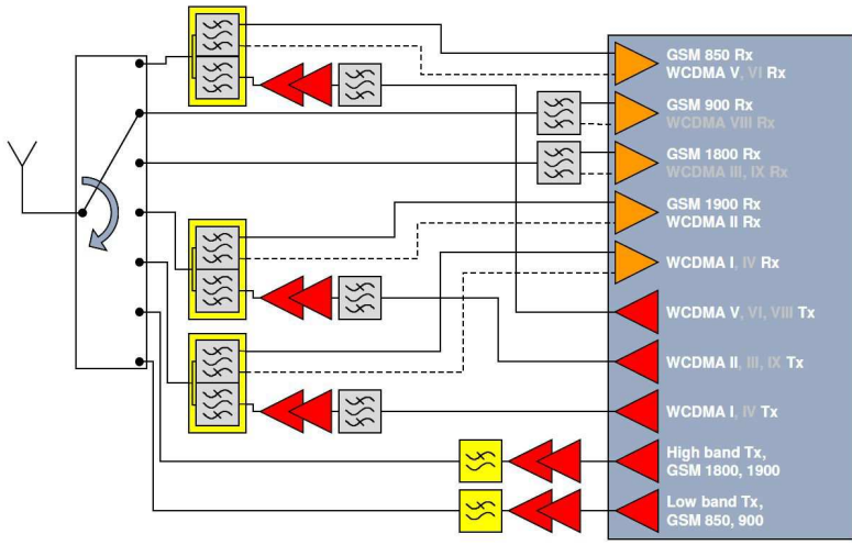
Multiband, multi-mode cellular phone [1].
