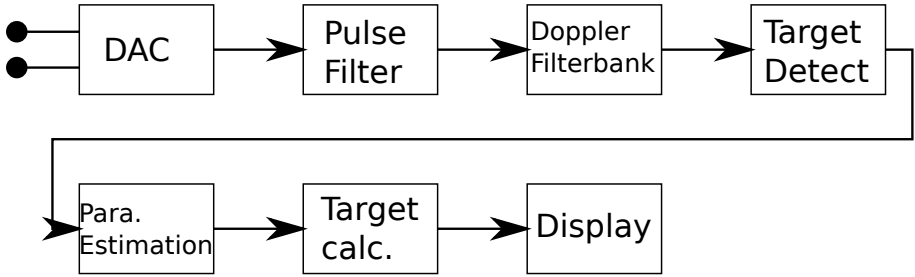
(Mostly) Digital part of a typical pulse Radar
