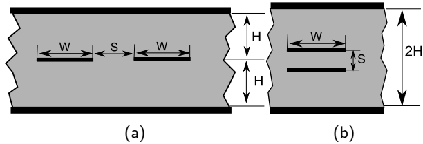
Coplanar (a) and broadside (b) coupled striplines
